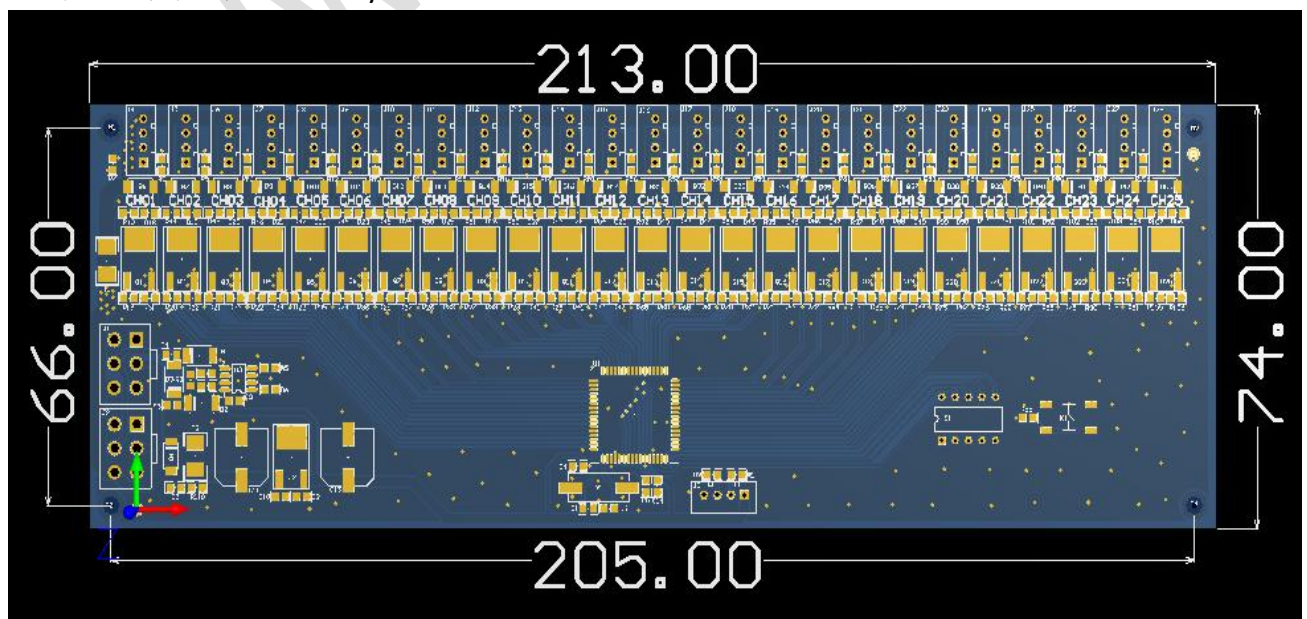
25 路锁控板尺寸图 25 way lock board size
