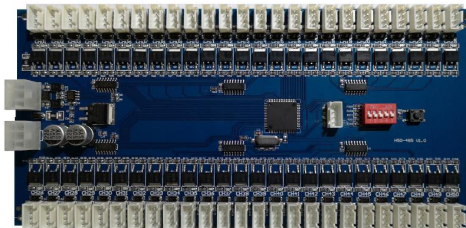
50 路锁控板 50way RS485 lock board:
