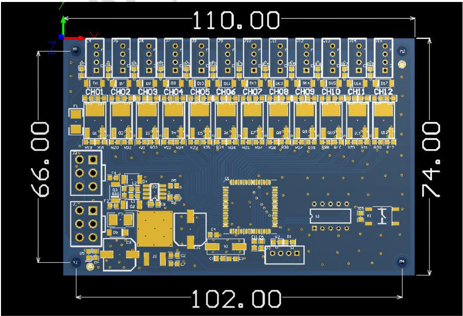
12 路锁控板尺寸图 12 way lock board size
